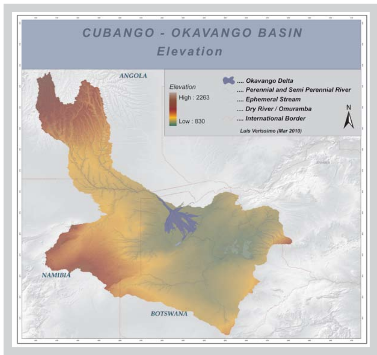
Figure 3.1: Cubango-Okavango Basin – elevation and topography
