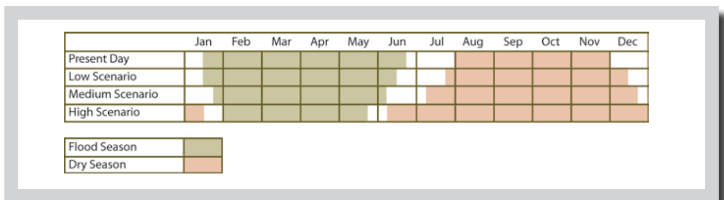
Figure 6.4: Changes in onset and duration of dry and flood seasons at Popa Falls and the panhandle under different scenarios. White areas are times of transitional flow between flood and dry seasons
