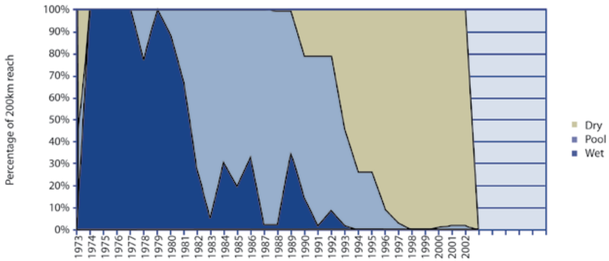
Figure 6.7: Percentage of the Boteti River study reach that will be inundated (wet); isolated pools (pool) and dry under the Low Scenario
