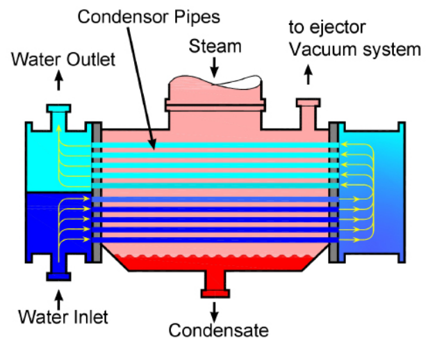
Figure 5 Condenser unit of thermal power plant
