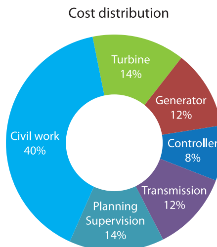
Figure 27 Average cost distribution of micro-hydro systems adopted from Indonesia experience (Source: Own diagram by Entec, 2011)
