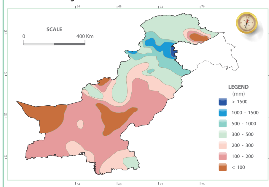
Figure 1. Mean Annual Rainfall in Pakistan
